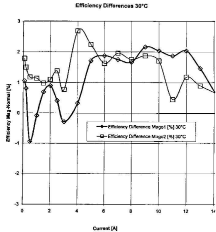
Figure 16: A reproduction of data from Ref. [45] showing the clear increase of the efficiency of a fuel cell when using Santilli MagneHydrogen with minimal increase of specific weight and conventional Oxygen.
