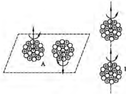
Figure 8: A generally ignored necessary condition for the proper coupling of nuclear spins as a necessary condition to avoid fusions at random and achieve them in a controlled fashion. According to the laws for nuclear syntheses set forth by hadronic mechanics, controlled nuclear syntheses can only occur for the "planar singlet coupling" in the left or the "triplet axial coupling" in the right [20].
