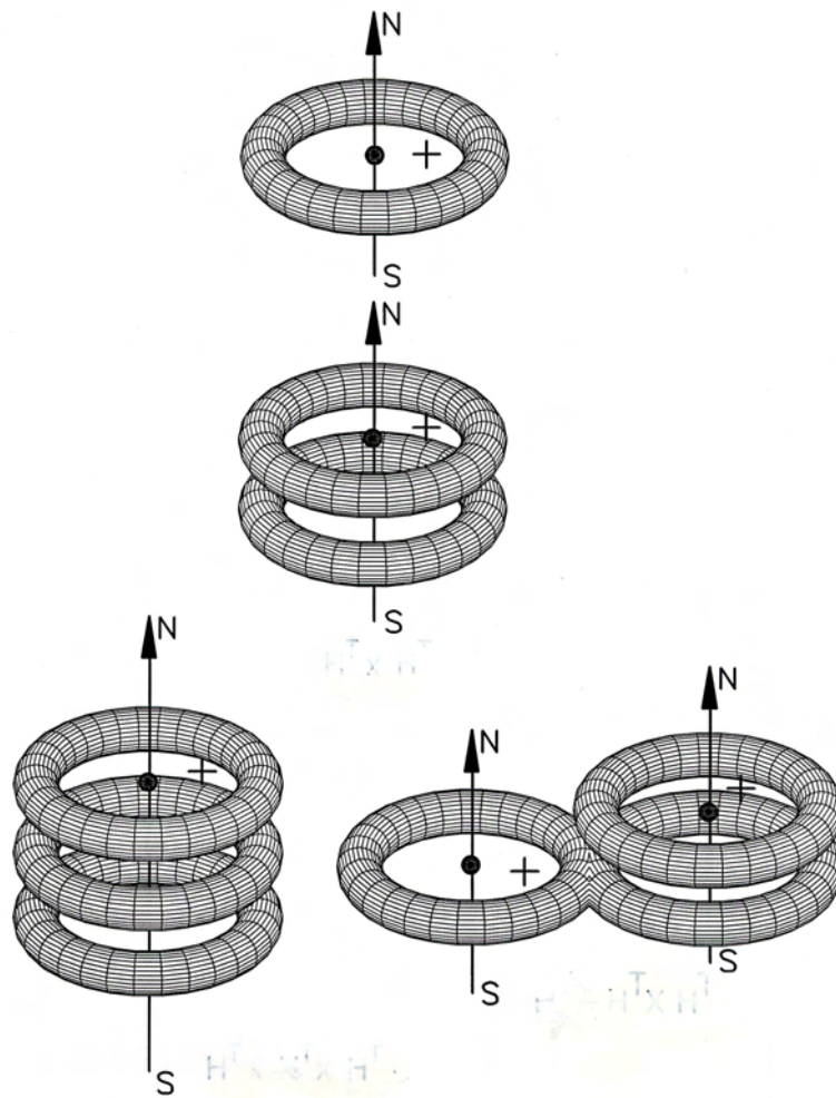
Figure 17: An artist rendering of the structure of Santilli magnequles in MagneHydrogen as a combination of Hydrogen atoms and molecule under the magnequcular bond.
