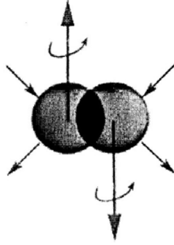
Figure 11: In the same way as quantum mechanics cannot be exactly valid for nuclear structure, Santilli has shows that quantum chemistry cannot be exactly valid for molecular structures because the two identical valence electrons in singlet coupling must repel each other according to quantum chemistry, while the covering hadronic chemistry has indeed achieved a strongly attractive force that overcomes the Coulomb repulsion [42-44].
