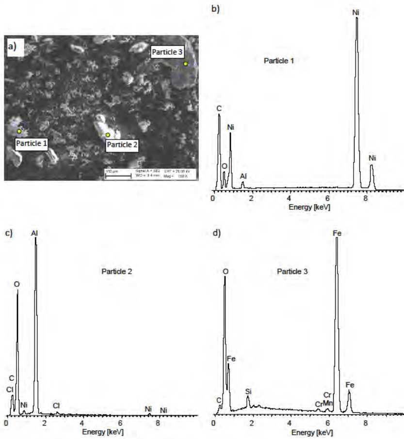
Figure 1: Reproduction of some of the scans from Appendix 3 of Ref. [2] establishing the existence beyond scientific doubt of nuclear transmutations with excess heat in Rossi's reactor that are beyond any quantitative interpretation via quantum mechanics.
