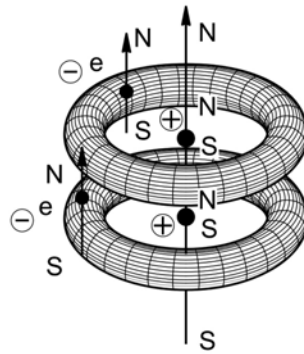
Figure 14: In Santilli’s view, an additional reason for the insufficient efficiency of various nuclear fusions at low energy is their lack of engineering realization of means for the systematic and controlled exposure of nuclei as an evident necessary prerequisite for the fusions themselves. Santilli constructed decades of research to solve this problem, including the construction of hadronic chemistry and the new chemical species of magnecules (here depicted) to achieve a controlled exposure of nuclei, as well as their proper spin alignment [42].
