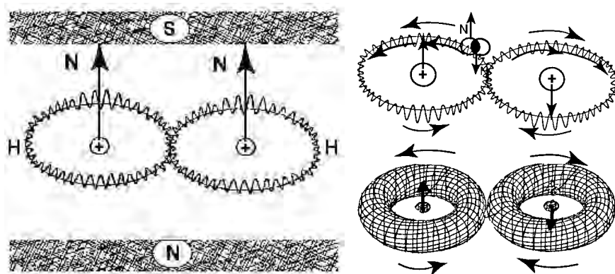
Figure 12: In the left, we illustrate another reason establishing the impossibility for quantum chemistry to be exactly valid for molecular structures, given by the prediction from the current treatment of orbitals that all quantities are paramagnetic in dramatic disagreement with experimental evidence [42]. In the right, we illustrates how the Santilli-Shillady strong valence bond assure the diamagnetic character of the Hydrogen and water molecules [43-44].
