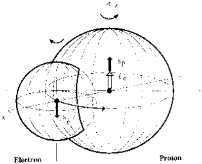
Figure 3: A basic novelty in Santilli's synthesis of the neutron from the Hydrogen atom is the appearance of a constrained angular motion of the electron immersed within the hyperdense proton. This orbital motion eliminates the need for the emission of a neutrino; it is solely permitted by the representation of the proton as extended according to hadronic mechanics; and it did not exist during Pauli's and Fermi's time since quantum mechanics solely represents the proton as a massive point [3-8].
