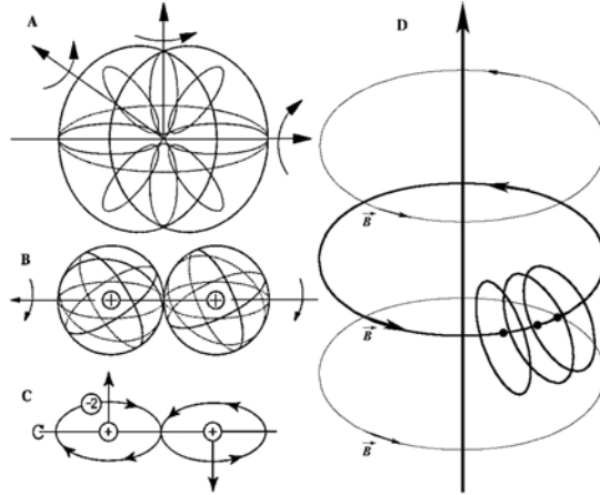
Figure 13: An illustration from Ref. [42] of the process according to which Santilli controls the orbit (rather than orbital) of the electron in the Hydrogen atom down to the desired toroid polarization.
