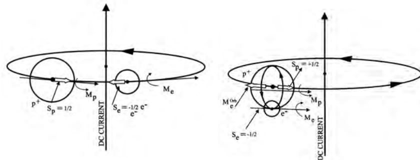
Figure 2: Schematic view of Santilli's synthesis of the neutron from the Hydrogen atom in the core of a star. The figure in the left depicts the ionization of the Hydrogen atom via an electric arc and the proper alignment of the proton and the electron. The figure in the right illustrates the coupling of the proton and electron at short distances. Additional contributions called the "trigger" force the penetration of the electron inside the hyperdense proton according to the laws of hadronic mechanics [3-8].
