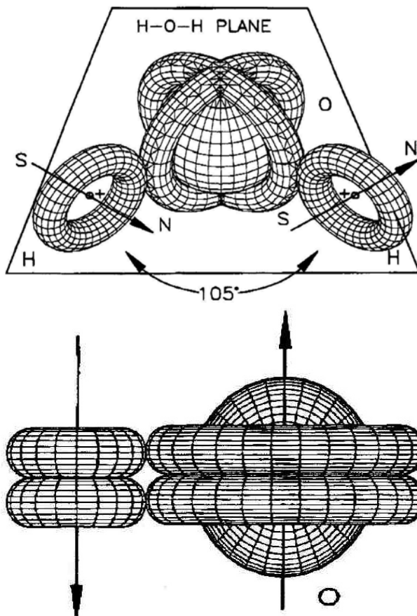
Figure 18: A suggestive conversion from Ref. [47] of liquid water (top) into a gaseous and combustible form Santilli calls HHO (bottom). The conversion is achieved via engineering means to remove the 105^\circ in between the two O - H dimers, in which case the l.h.s. form is turned into the r.h.s. one with chemical structure (H \times H) - O , where - denotes valence bond and \times denotes magnetic bond. The new species (H \times H) - O is clearly gaseous, because of the lack of the covalence bonds for the liquid state, besides the fact that the Hydrogen is much lighter than the Oxygen molecule. Also, the structure (H \times H) - O is unstable, thus decaying into a stoichiometric mixture of Santilli MagneHydrogen H \times H and Oxygen O - O that instantly melts bricks without any need for oxygen, thus confirming the special feature of Santilli Magnehydrogen.
